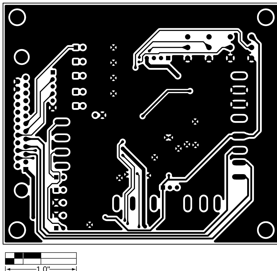
Figure 4. MAX769 EV Kit PC Board Layout—Solder Side
