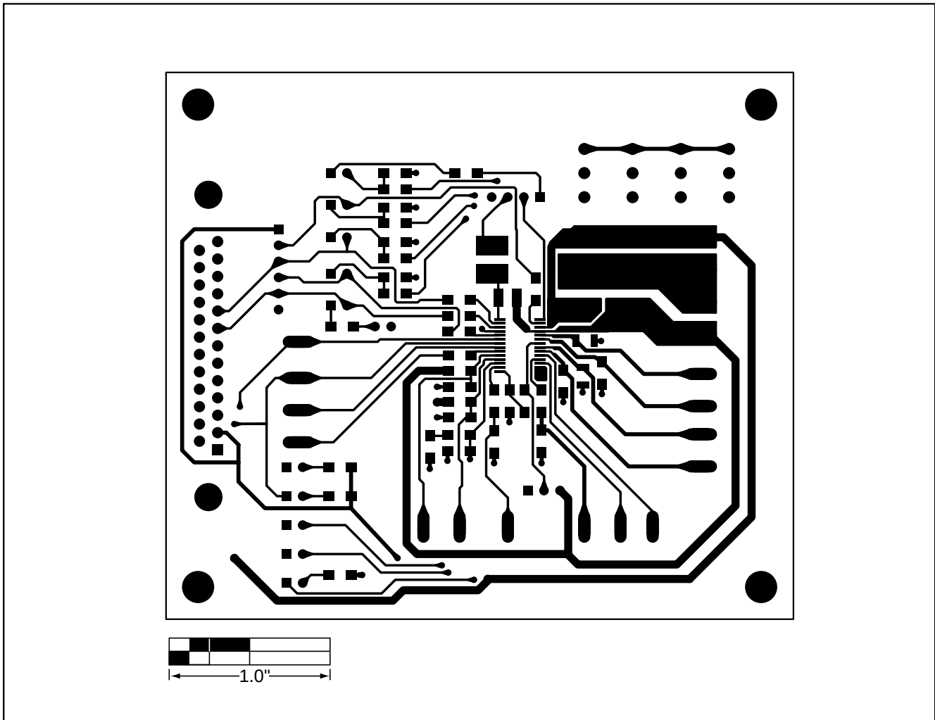
Figure 3. MAX769 EV Kit PC Board Layout—Component Side
